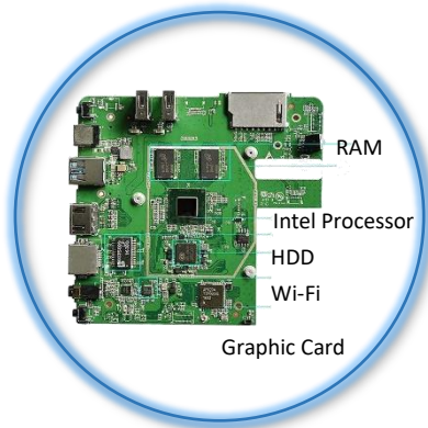
SBC – Single Board Computer
